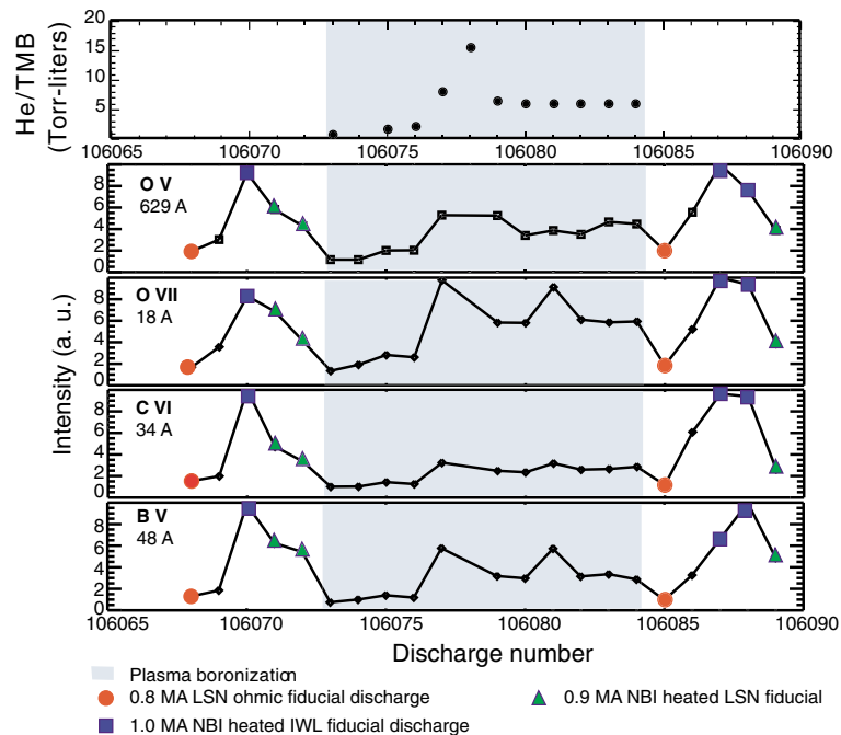
Fig. 3. The 90% He–10% TMB fueling discharge sequence (top), and oxygen, carbon, and boron luminosities. The clean initial edge conditions were only marginally improved. Edge fueling with TMB did not increase B V and C VI.
