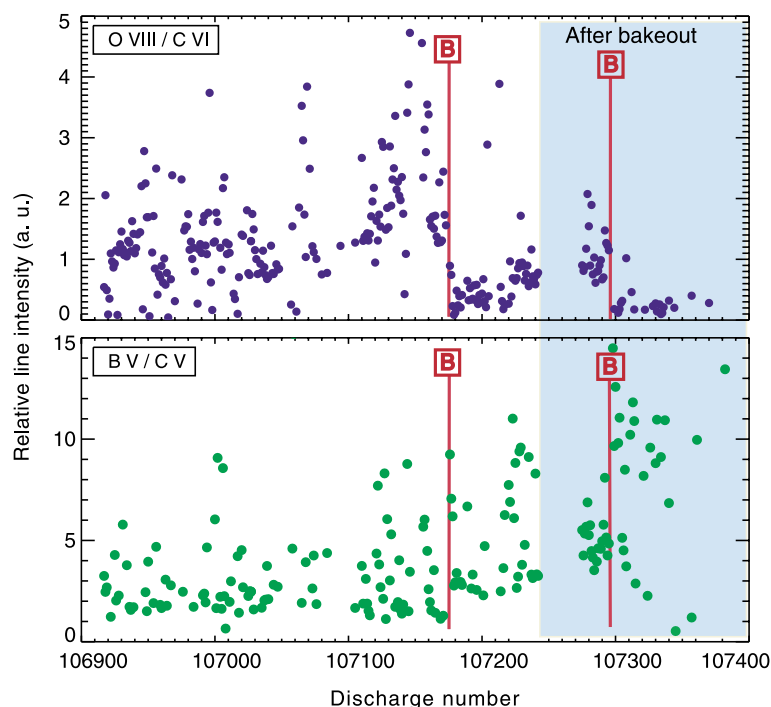
Fig. 2. Relative intensities of O VIII/C VI (top) and B V/C V (bottom) for discharges before and after bake-out and subsequent boronization.
