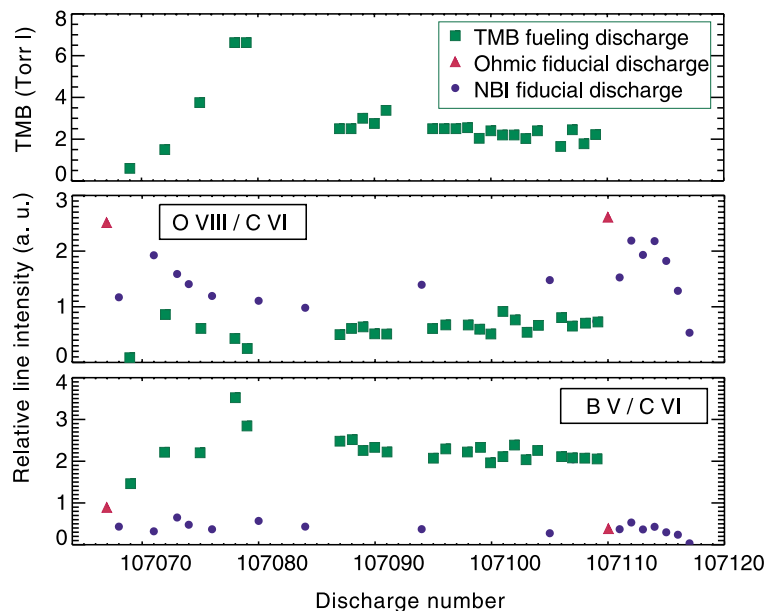
Fig. 4. The TMB (100%) fueling discharge sequence (top), and the oxygen, carbon, and boron relative intensities.
