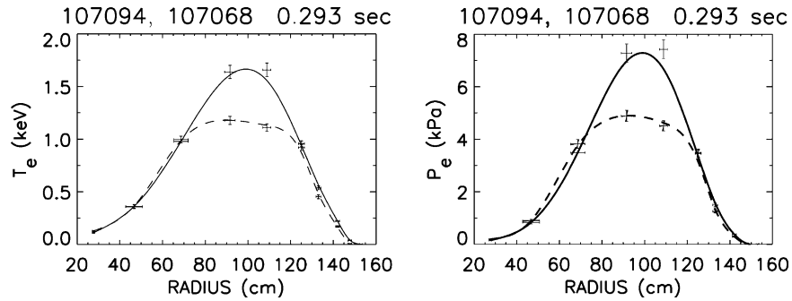
Fig. 5. Comparison of electron temperature, and pressure profiles for one of the highest central electron temperatures, T_e(0) \sim 1.6 keV achieved in NBI heated discharges observed in a fiducial discharge following a TMB fueling sequence (solid), and a fiducial discharge of the same density before TMB fueling started (dashed).
