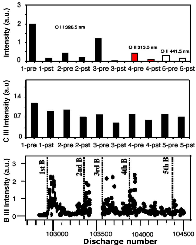
Fig. 1. Oxygen and carbon luminosities for boronizations 1 through 5. GDC boronization with deuterated TMB consistently reduced oxygen and carbon. The results are most comparable for a given boronization because some change in the fiducial discharges occurred between boronizations.
